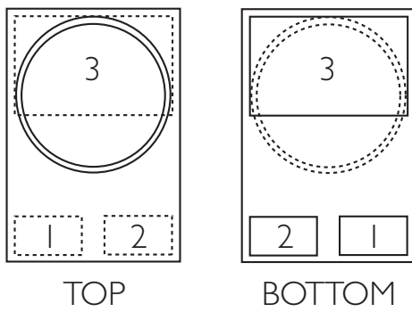
Figure 9a. LUXEON Rebel Color Line pad configuration.
